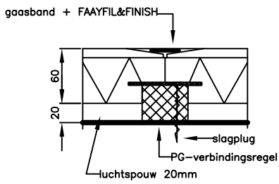
koppeling PG60 system
