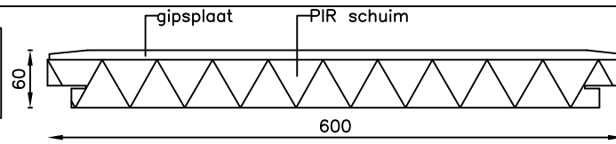
PG60 system AK
