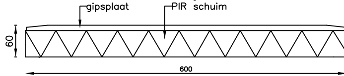
PG60 Basic AK
