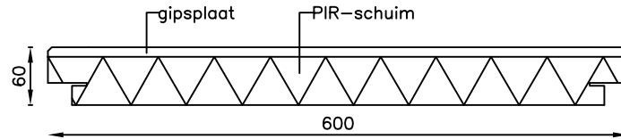
PG60 system FK
